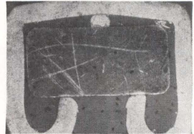
MICROSECTION shows wire being held onto post by spring action of terminal
