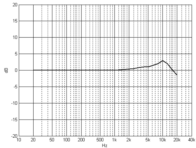
N101/N101-Pair Frequency Response
