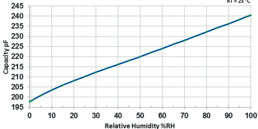
Characteristics HT-1
