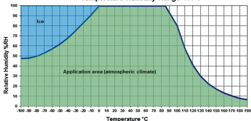
Temperature-Humidity-Range HT-1
