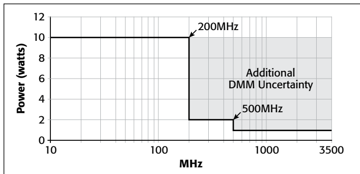
Figure 2. Carry power per channel vs. frequency for the Model 7711 switch module.
