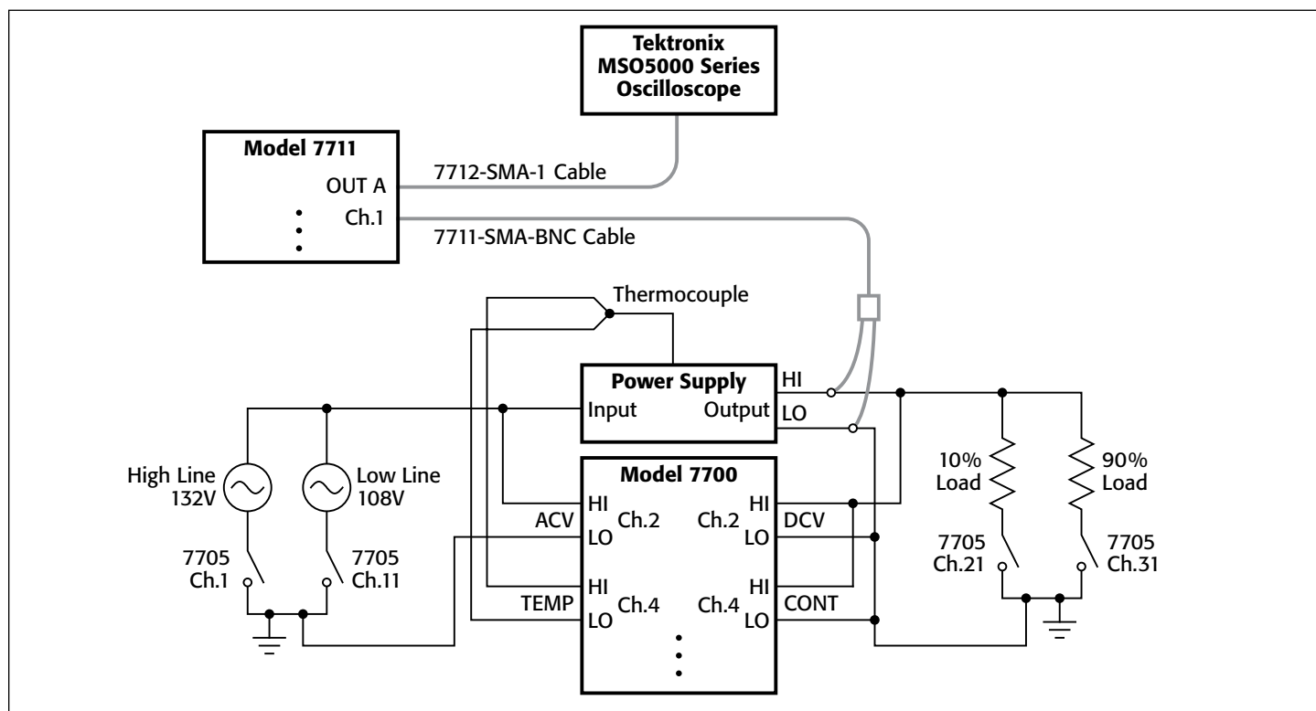
Figure 1. DC power supply test diagram. Only one power supply is shown; additional switching channels would be used to connect multiple supplies to the measuring instruments.
