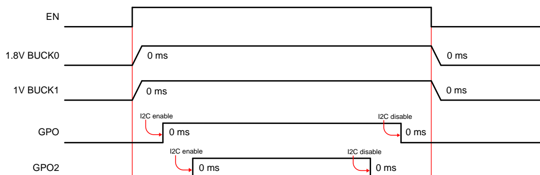
Figure 1. TPS6565342-Q1 Power-up and Power Down Sequence
