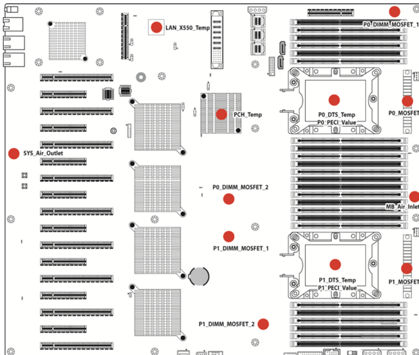
Figure 1: Sensor Location
