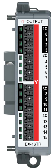
BX-16TR Output Module 16-pt, Relay Form A (SPST)
