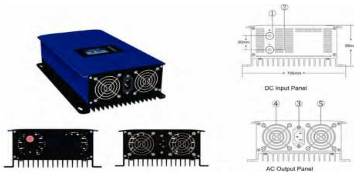
Fig 14 SUN-2000G2-X-X
