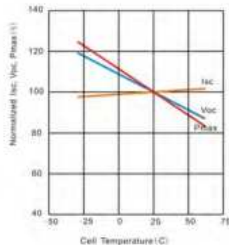
Fig 3. Temperature Dependence of Isc, Voc, Pmax
