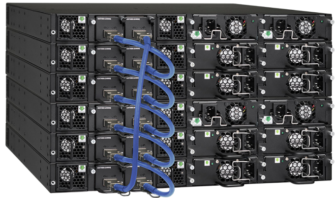
Figure 1: RUCKUS ICX switches can be stacked together using standard SFP+ or QSFP+ ports and optics to create a single logical device over distances up to 10 km.
