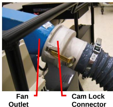
Figure 6. Positive Pressure, High-Flow Set-Up
