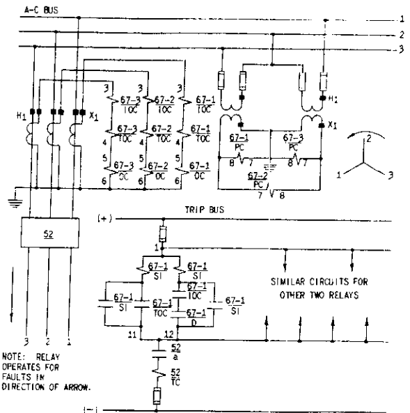
* Fig. 7 Internal Connections for Type JBC78E Relay (Front View)
