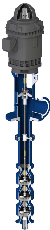
VIT/DWT lineshaft
