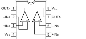
IC581 : TK15420M Video Amp
