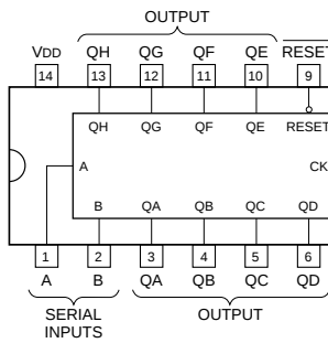
IC586 : TC74HC164AF-EL 8-Bit Shift Register
