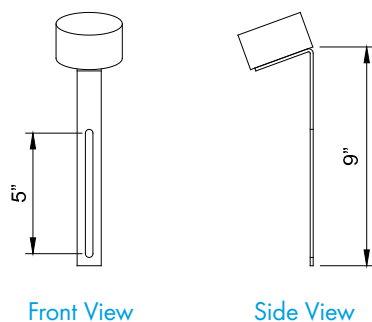
COUNTERWEIGHT, AC1512
