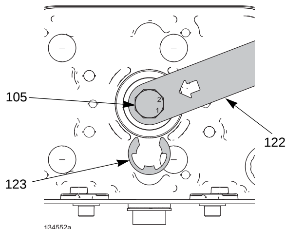
FIG. 8 Stroke adjustment - lever arm positions
