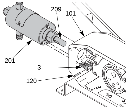
FIG. 10 Disconnect the fluid cylinder
