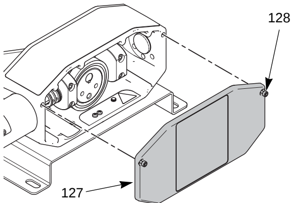
ti34755a FIG. 9 Expose the drive shaft
