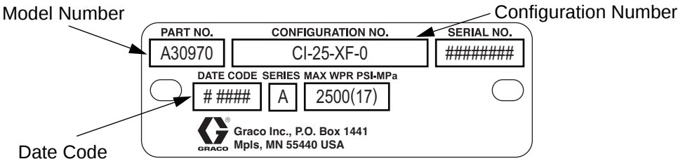
FIG. 2 Example of the Fluid Module Identification Plate
