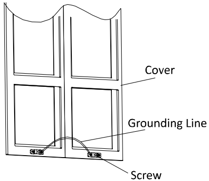
Figure 3-55 Connect the Grounding Line to the Cover
