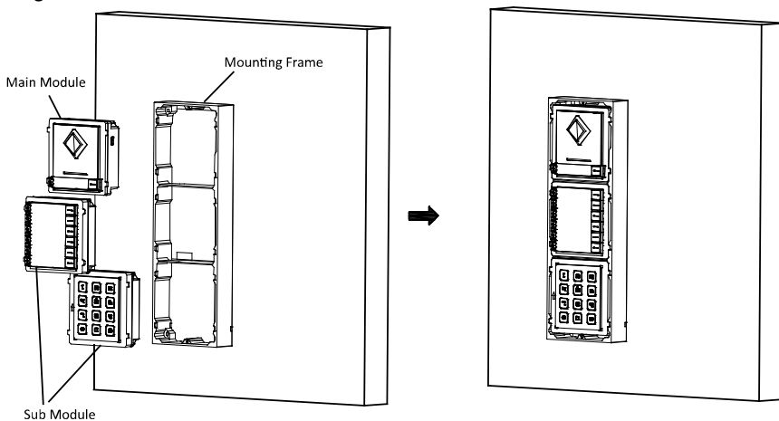
Figure 3-38 Insert the Modules
