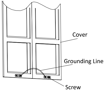
Figure 3-68 Connect the Grounding Line to the Cover
