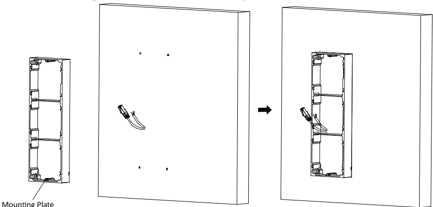
Figure 3-35 Fix the Mounting Frame
