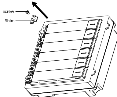
Figure 3-2 Remove the Screw and Shim
