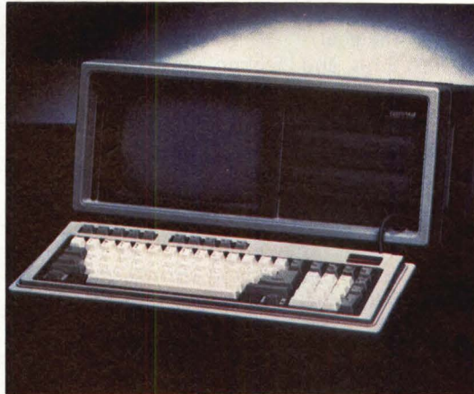
Supporting up to 4M bytes of internal RAM memory, the Compaq Portable II uses a 6-MHz 80286 and operates as a single-user workstation.
