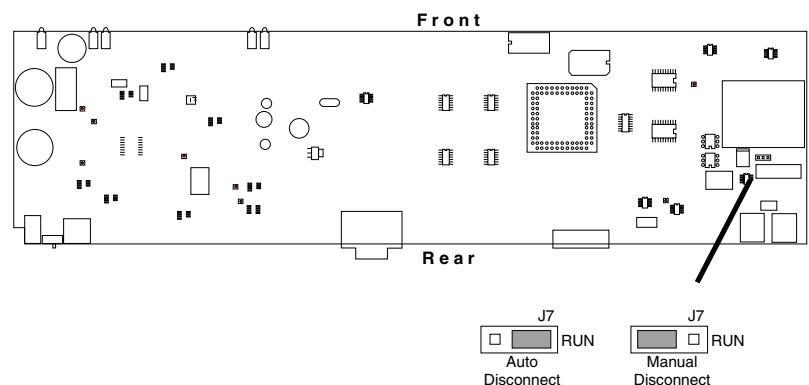
Figure 10 - Location of DC Bypass Jumper
