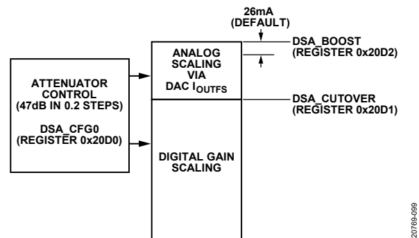
Figure 110. DAC I_{OUTFS} and Digital Gain Controlled by Look Up Table
