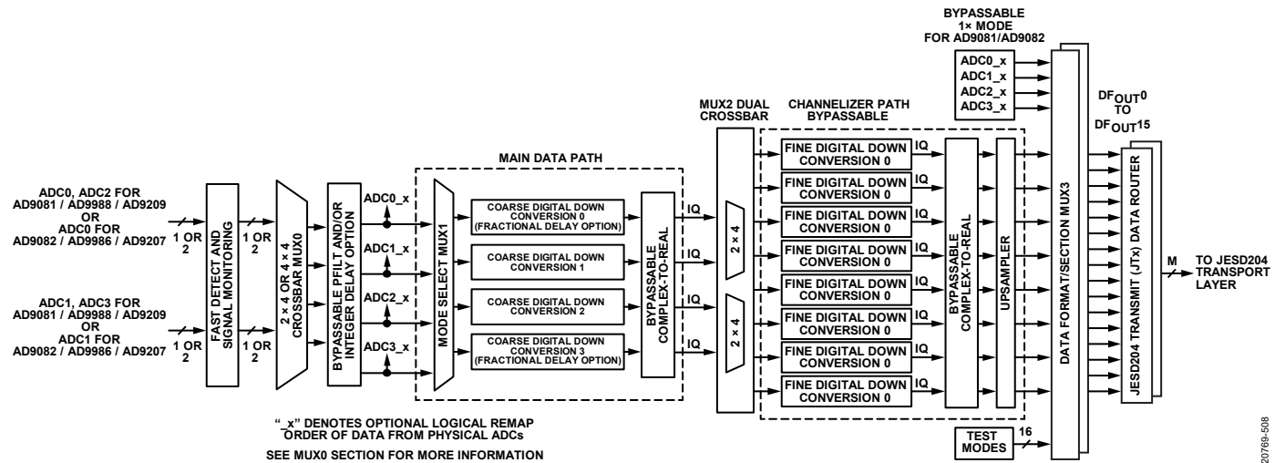
Figure 37. Complete Receive Digital Data Path
