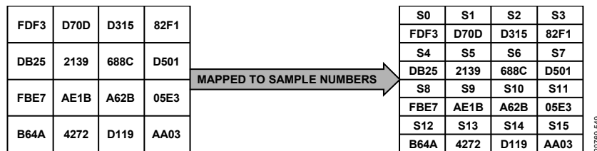
Figure 152. First 16 16-bit PRBS7 Samples Mapped to Converter Sample Number
