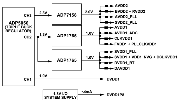
Figure 146. Suggested Power Delivery Network
