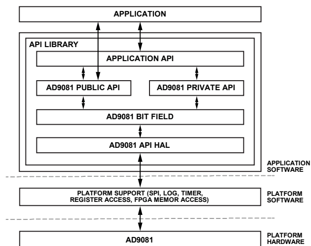
Figure 3. AD9081 API Architecture
