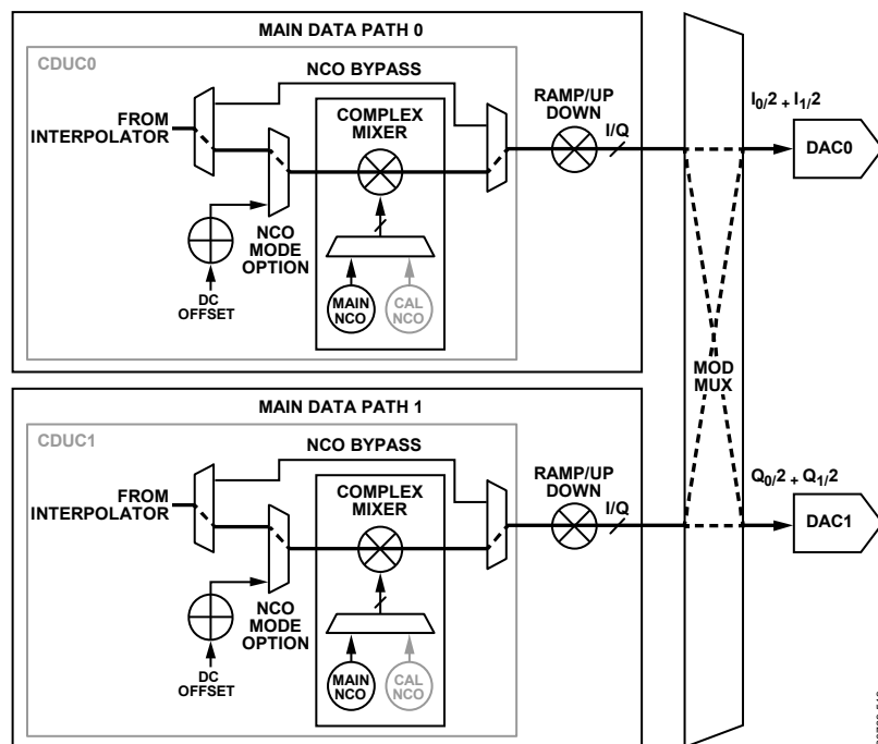
Figure 81. Mod Mux Configuration 3A, EN\_CMPLX\_MOD = 1 , all NCOs Enabled— DAC0 = (I_0 + I_1)/2 , DAC1 = (Q_0 + Q_1)/2
