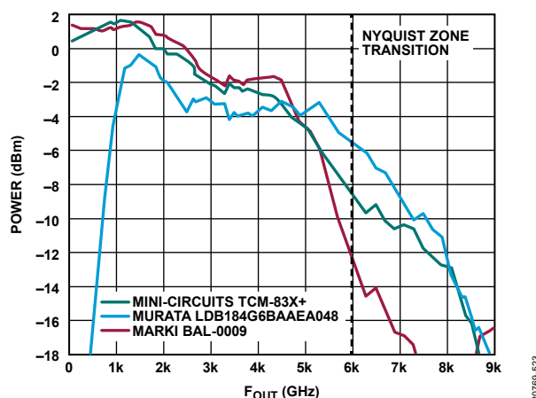
Figure 88 DAC Frequency Response with 12 GSPS Update Rate for Different Baluns with Optimized PCB Layouts
