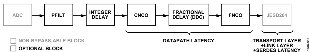
Figure 118. Latency Block Diagram
