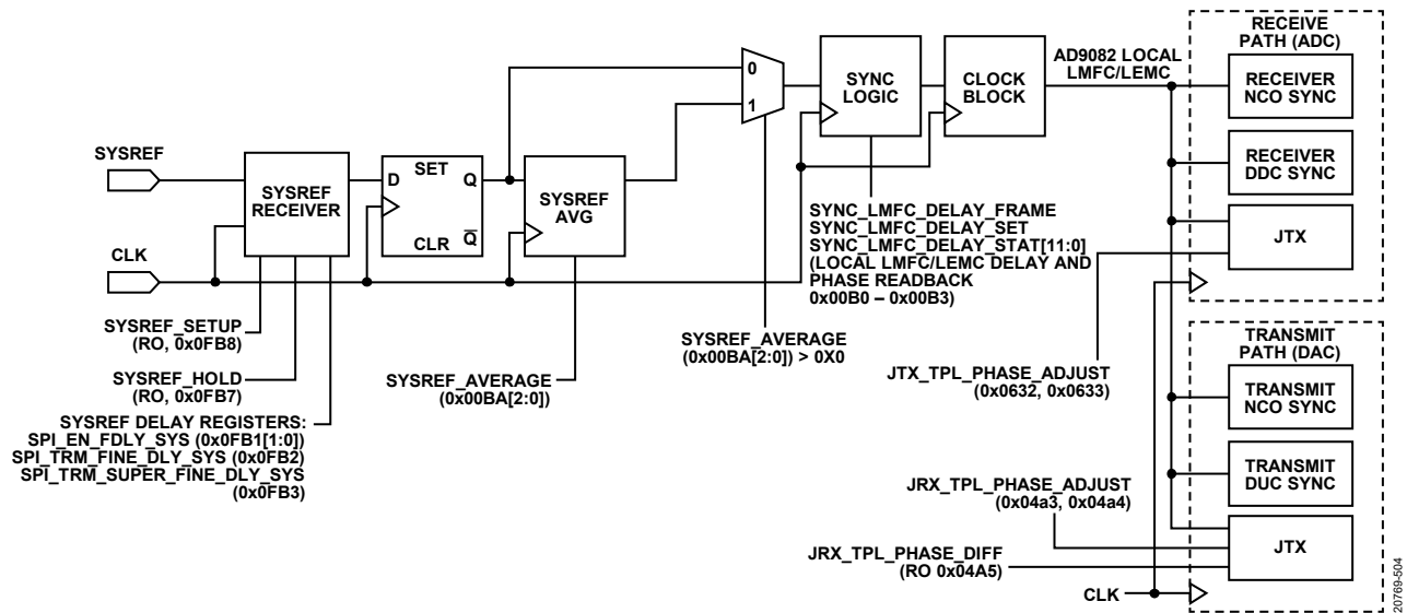
Figure 20. Chip Level Synchronization Block Diagram
