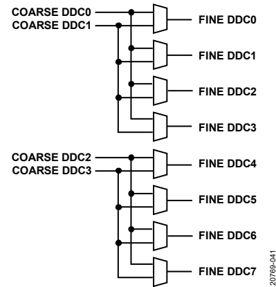
Figure 45. Dual 2×4 Crossbar Multiplexer
