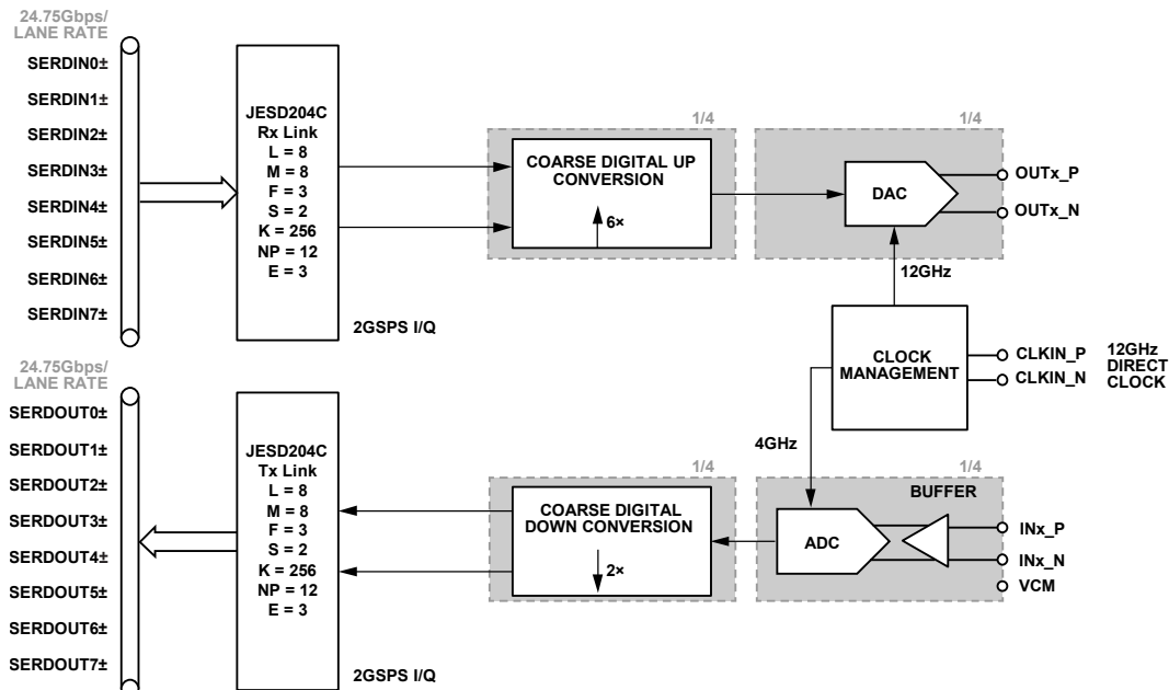
Figure 141. 4D4A, DAC in 2 GSPS I/Q Mode, ADC in 2 GSPS I/Q Mode Block Diagram
