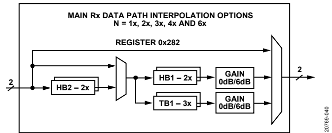
Figure 44. Main Datapath Decimation Filter Lineup
