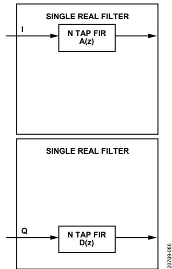
Figure 99. Single Real Coefficient FIR Filter on the I or the Q channel
