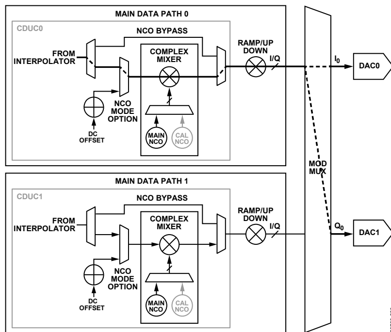
Figure 82. Mod Mux Configuration 3B, EN\_CMPLX\_MOD = 1 , NCO of CDUC1 Disabled— DAC0 = I_0 , DAC1 = Q_0
