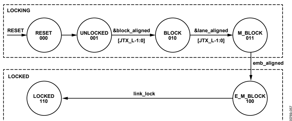
Figure 62. JESD204C Receiver Synchronization State Diagram
