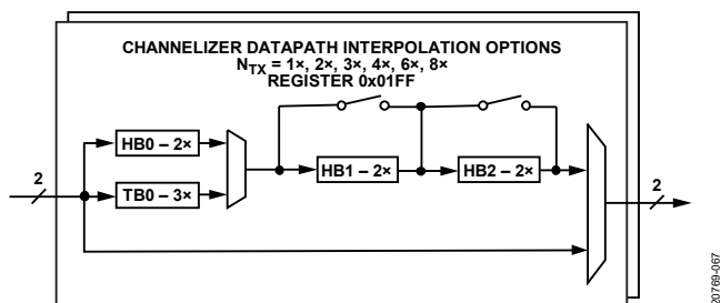
Figure 72. Channelizer Interpolation Filter Lineup
