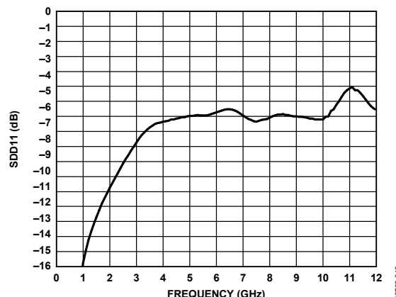
Figure 15. Clock Receiver Differential Input Return Loss
