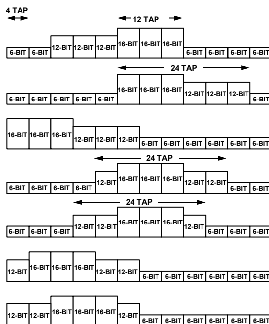
Figure 106. PFILT Coefficient Size Examples
