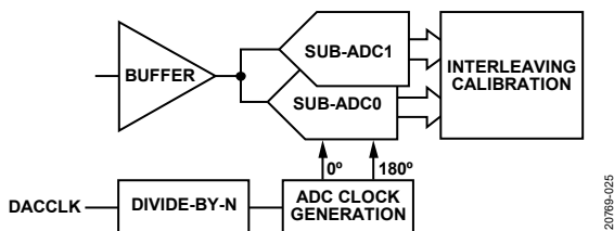
Figure 27. ADC Architecture of AD9081 4 GSPS ADC
