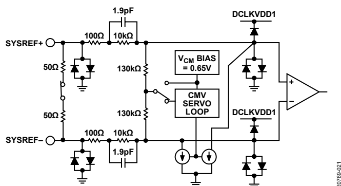
Figure 21. SYSREF \pm Receiver Block Diagram
