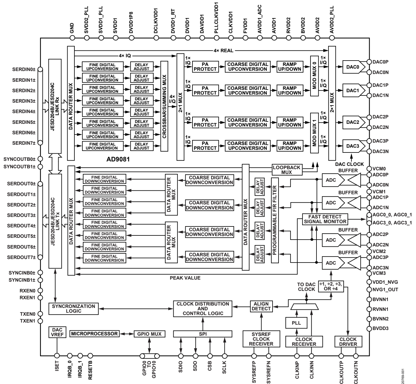
Figure 1. AD9081 Functional Block Diagram
