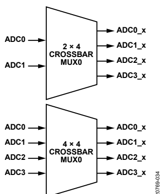
Figure 38. 2×4 and 4×4 Crossbar Mux0 for AD9082 and AD9081
