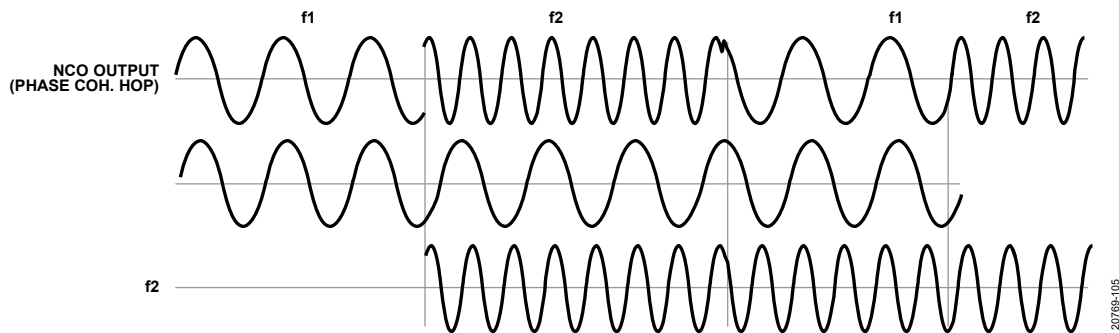
Figure 116. Transmit/Receive NCO FFH
