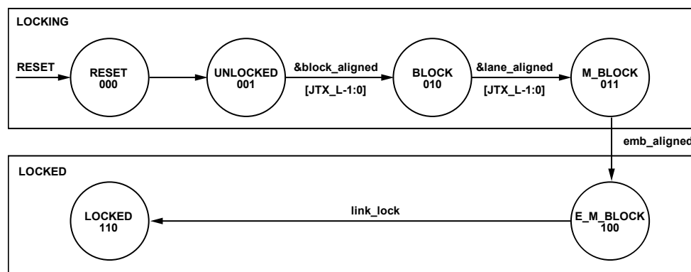
Figure 154. Flow Chart Showing Readback Values of Bits[6:4] of Register 0x055E
