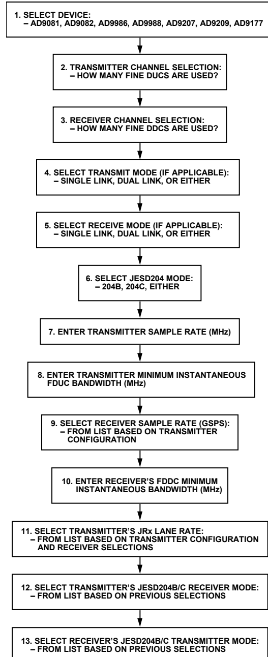
Figure 58. JESD204B/C Mode Selector Flow Diagram
