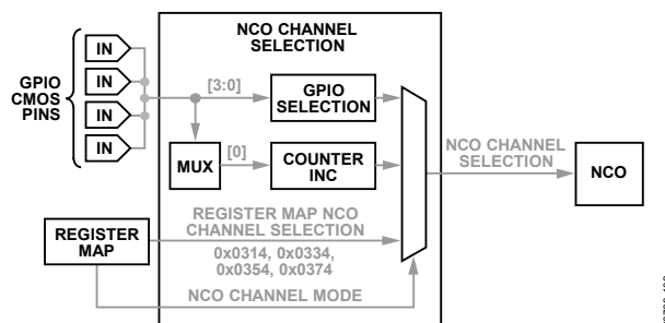
Figure 113. NCO Channel Selection Block
