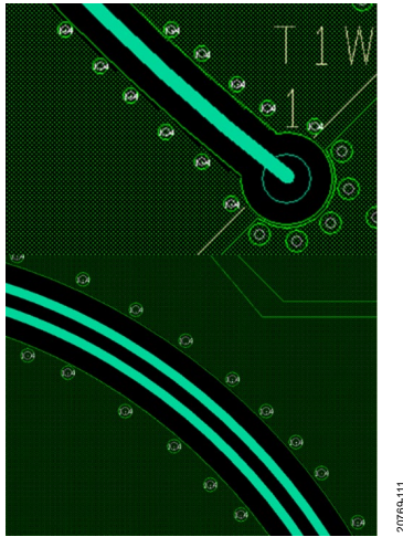
Figure 124. Fencing Technique on RF Analog (Top) and SERDES Lane Pairs (Bottom)
