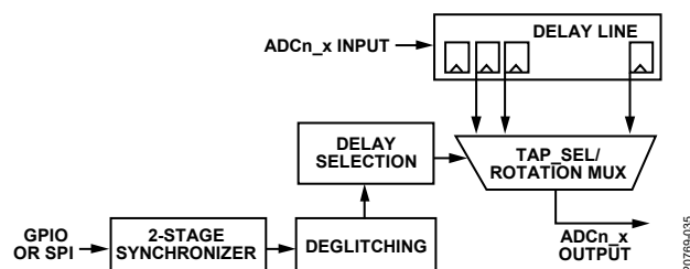
Figure 39. Optional Integer Delay Block Implementation
