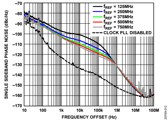
Figure 11. Single Sideband Phase Noise vs. Frequency Offset for Different PLL Reference Clock ( f_{REF} ), Output Frequency ( f_{OUT} ) = 1.8 GHz, f_{DAC} = 12 GSPS, PLL Enabled with Exception of External 12 GHz Clock Input with Clock PLL Disabled
