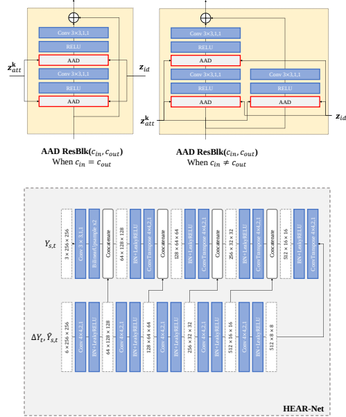
Figure 12: Network structures. Conv k,s,p represents a Convolutional Layer with kernel size k , stride s and padding p . ConvTranspose k,s,p represents a Transposed Convolutional Layer with kernel size k , stride s and padding p . All LeakyReLUs have \alpha = 0.1 . AAD ResBlk(c in , c out ) represents an AAD ResBlk with input and output channels of c_{in} and c_{out} .
