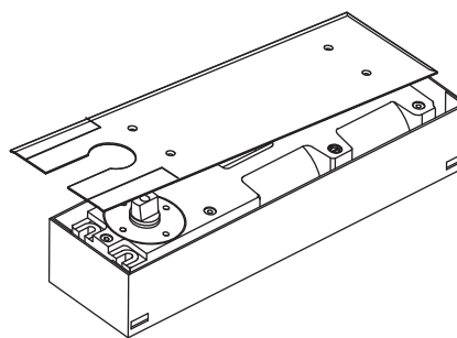
Standard Duty Floor Closer (FC-6280)
