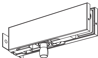
Transom Patch with Wall Bracket (PFT-34)
