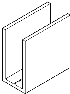
Wet/Dry U-Channel (UWD-2000x1000)
