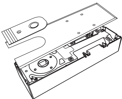
Standard Duty Floor Closer (FC-6275)
