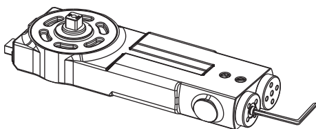
Rixson Overhead Closer (OHC-609)
