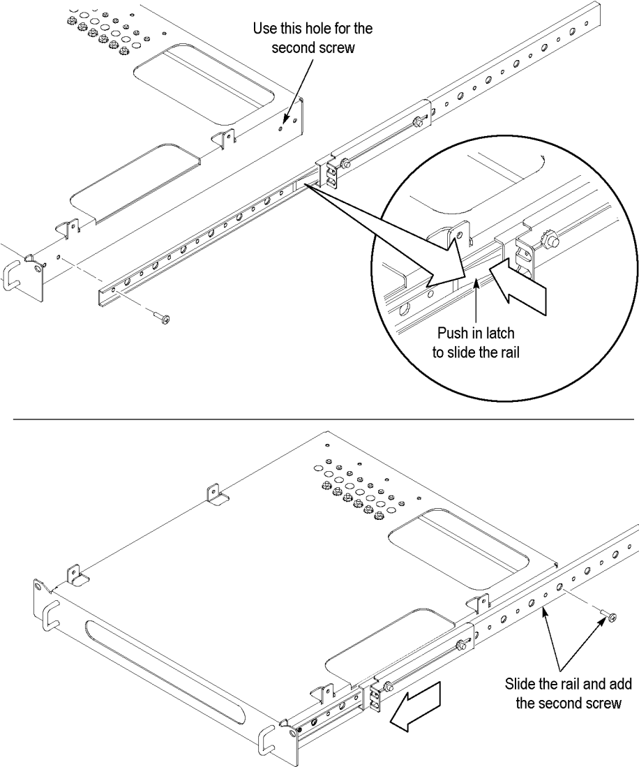
Figure 7: Rackmount shelf preassembly
