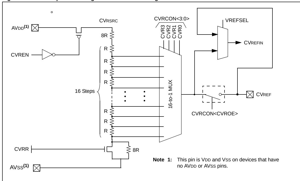
Figure 48-7: Comparator Voltage Reference Block Diagram
