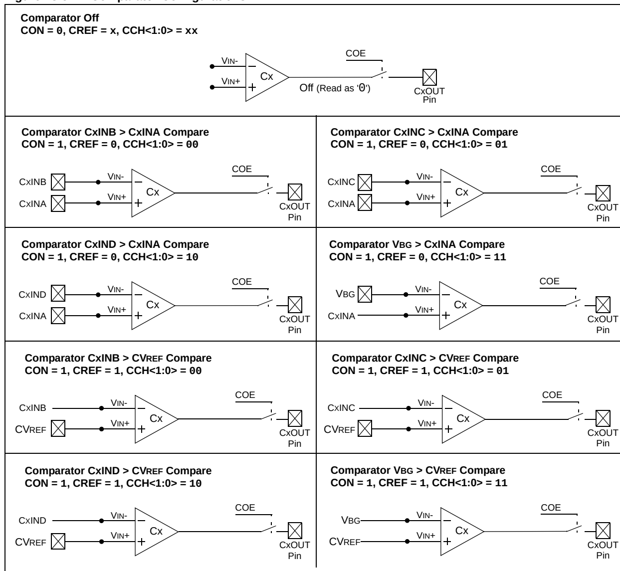
Figure 48-5: Comparator Configurations
