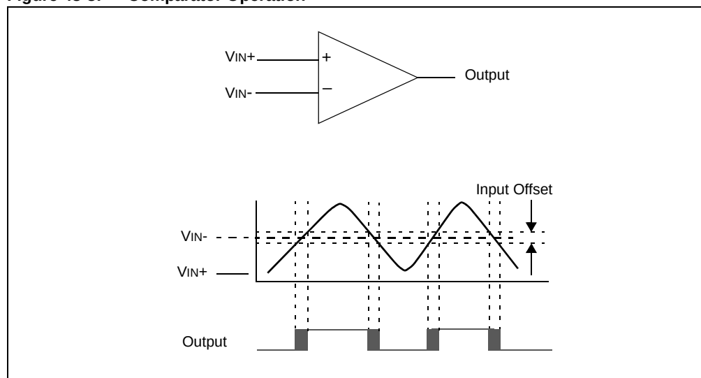
Figure 48-3: Comparator Operation
