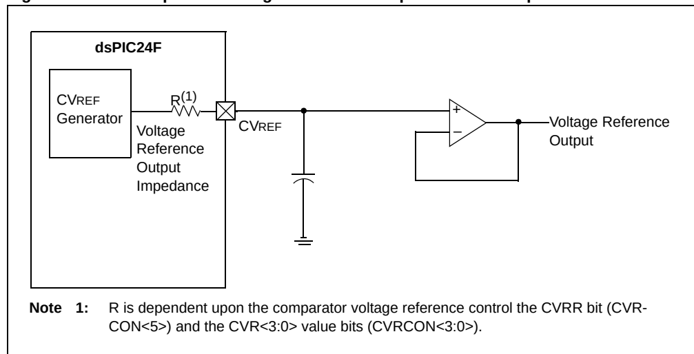
Figure 48-8: Comparator Voltage Reference Output Buffer Example
