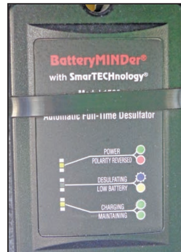
Figure 9-8: Battery maintainer
