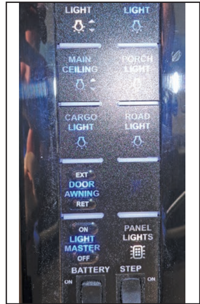
Figure 11-6: Entrance step switch
