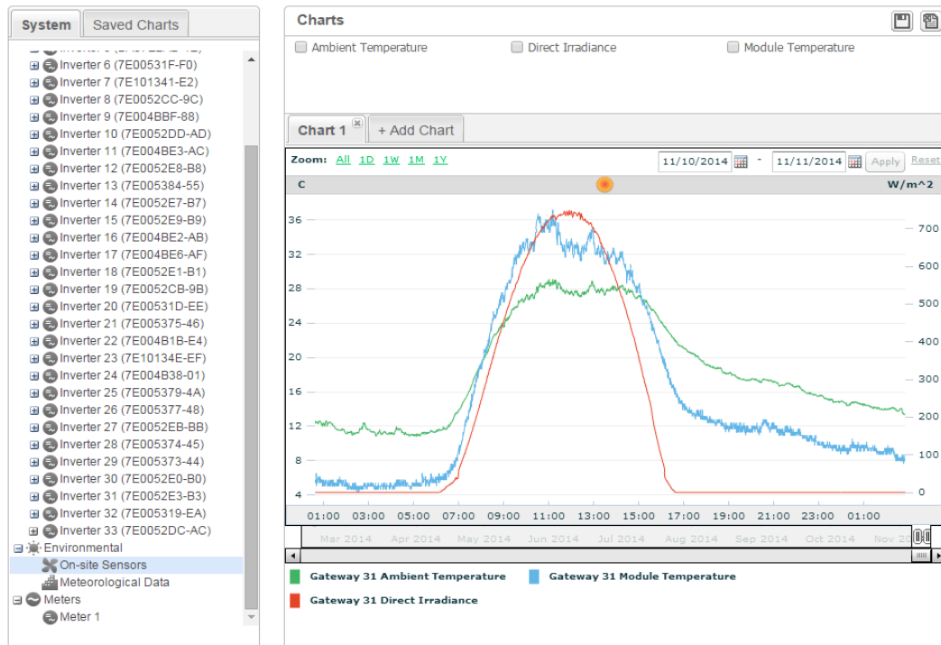
Figure 10: Viewing sensor readings on the monitoring platform
