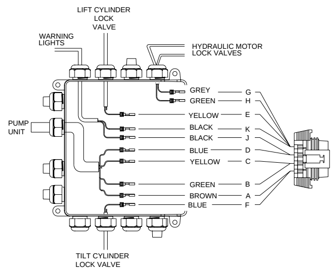
10- POLE CONNECTOR
