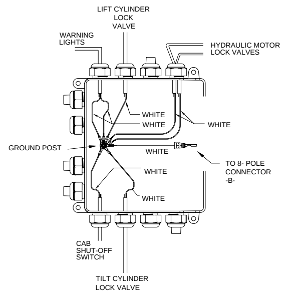
GROUND WIRE CONNECTIONS
