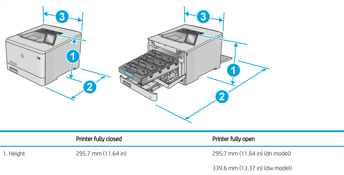
Figure 1-2 Dimensions for the M452dn and M452dw models
