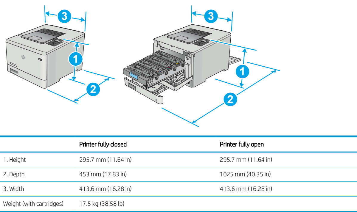
Figure 1-1 Dimensions for the M452nw model
