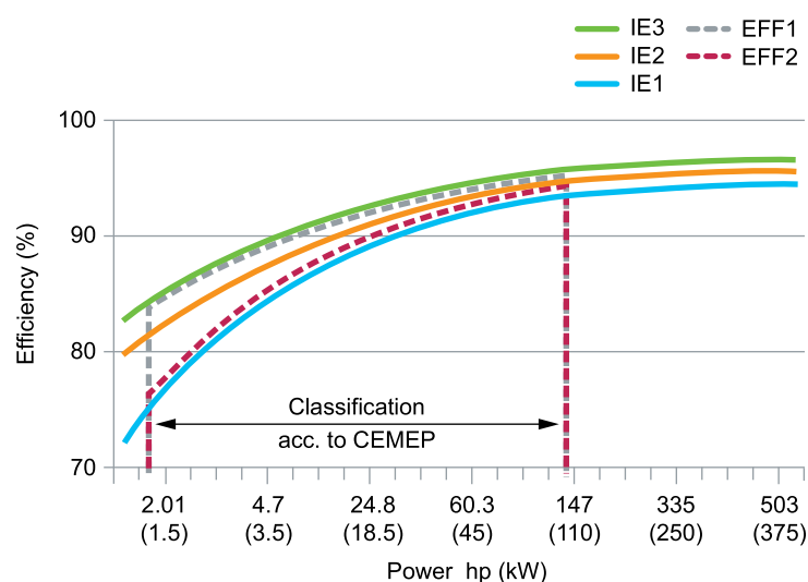
Figure 2 - Comparison of IE1, IE2, and IE3 Motors to EFF1 and EFF2 Predecessors
