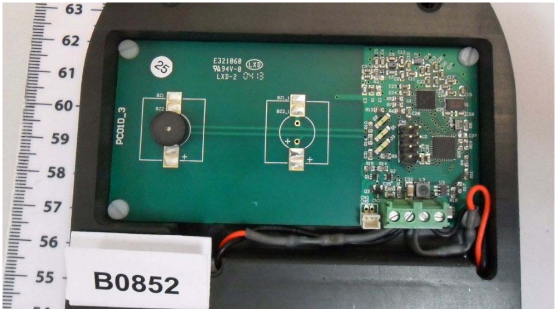
PCB and fuses
