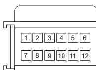
12 PINS male AMP connector contact insertion view
