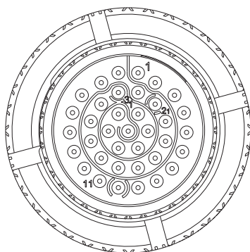
37 PINS female Deutsch connector contact insertion view
