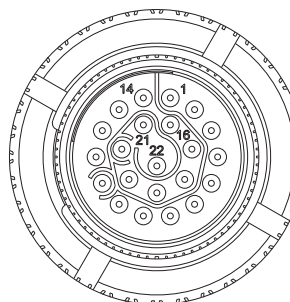
22 PINS female Deutsch connector contact insertion view
