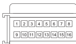
16 PINS male AMP connector contact insertion view
