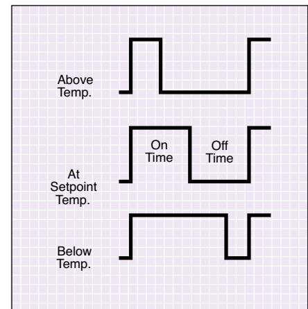
Figure 1: Proportional control
