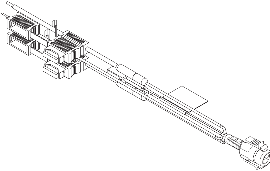
Figure 2-46. HKN6188_ Power Cable with External Speaker Connector
