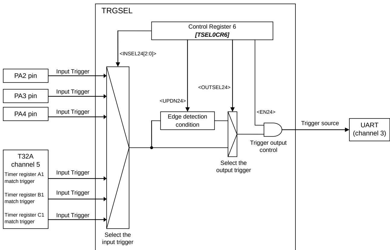
Figure 2.1 Example of Trigger Selector Connection
