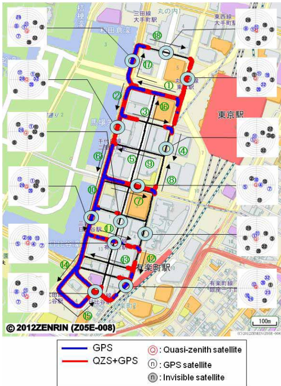
Fig. 7 Arrangement of satellites used for positioning at various locations en route
