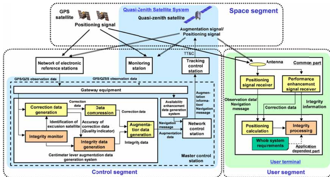
Fig. 1 Configuration of positioning system using QZS
