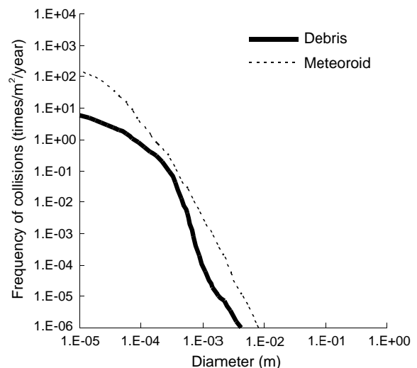
Fig. 4 Space debris environment around geostationary orbit satellites
