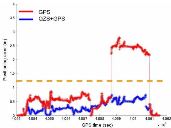
Fig. 8 Accuracy improvement by reduced multipath effects
