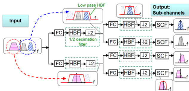
Fig. 3 Functional block diagram of demultiplexer
