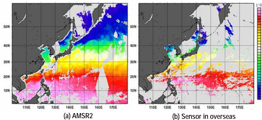
Fig. 3 Comparison of distribution of sea surface temperatures (Source: JAXA/JMA)
