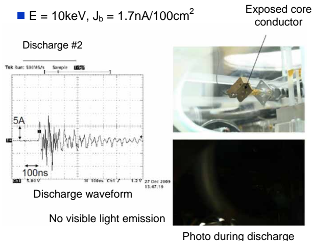
Fig. 5 Electrostatic charge/discharge test
