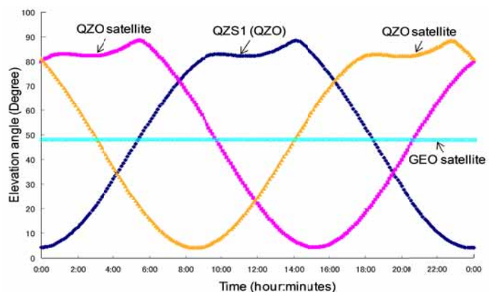
Fig. 3 Elevation angles of quasi-zenith satellites viewed from Tokyo
