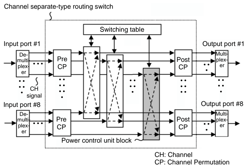
Fig. 6 Configuration of channel-separate-type routing switch
