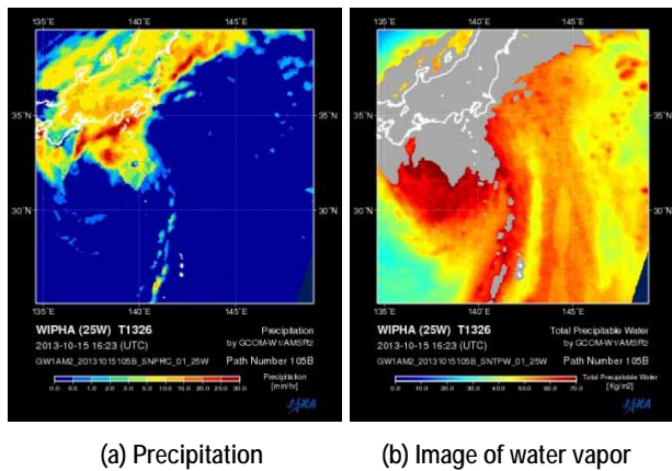
Fig. 2 Real-time monitoring of Typhoon No. 26 by AMSR2 data (Source: JAXA)
