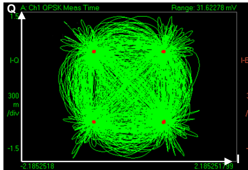
Fig. 7 Constellation of channelizer output signal
