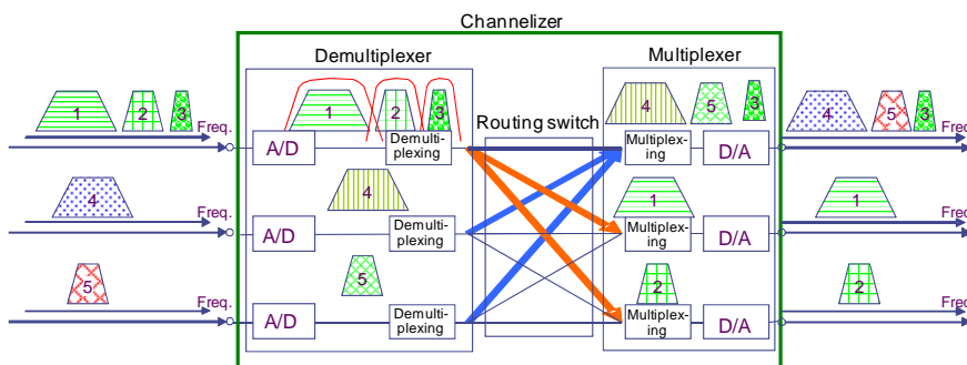
Fig. 1 Functional block diagram of channelizer
