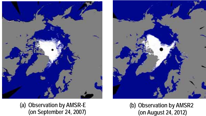
Fig. 5 Distribution of sea ice in the Arctic (Source: JAXA)
