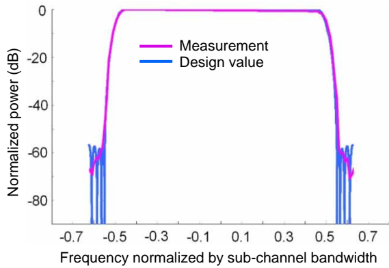
Fig. 5 Frequency characteristics of sub-channel filter
