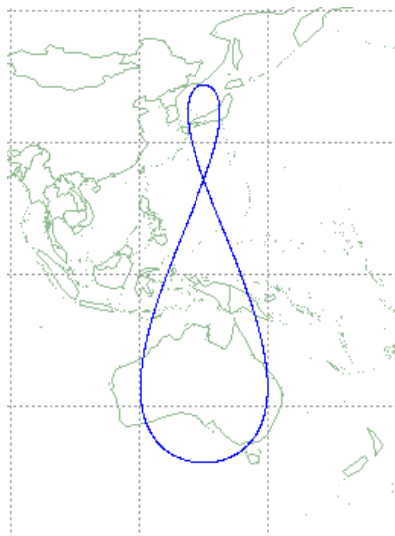
Fig. 2 Trajectory of quasi-zenith satellite projected onto the earth's surface (from IS-QZSS (1) )
