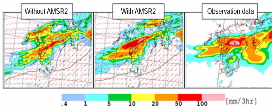
Fig. 4 Projection of precipitation distribution (Difference between with and without AMSR2 data) (Source: JAXA/JMA)
