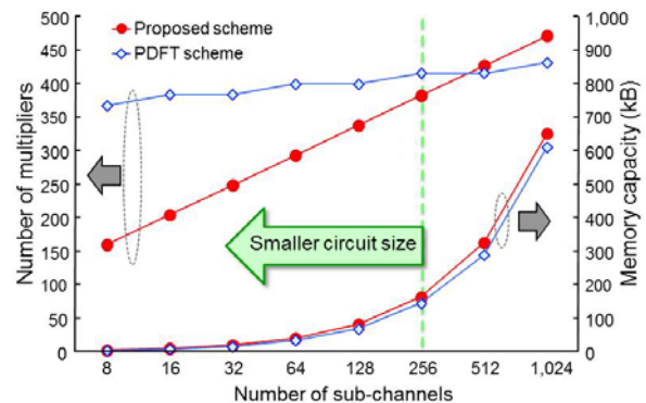
Fig. 4 Number of multipliers and memory capacity vs. the number of sub-channels
