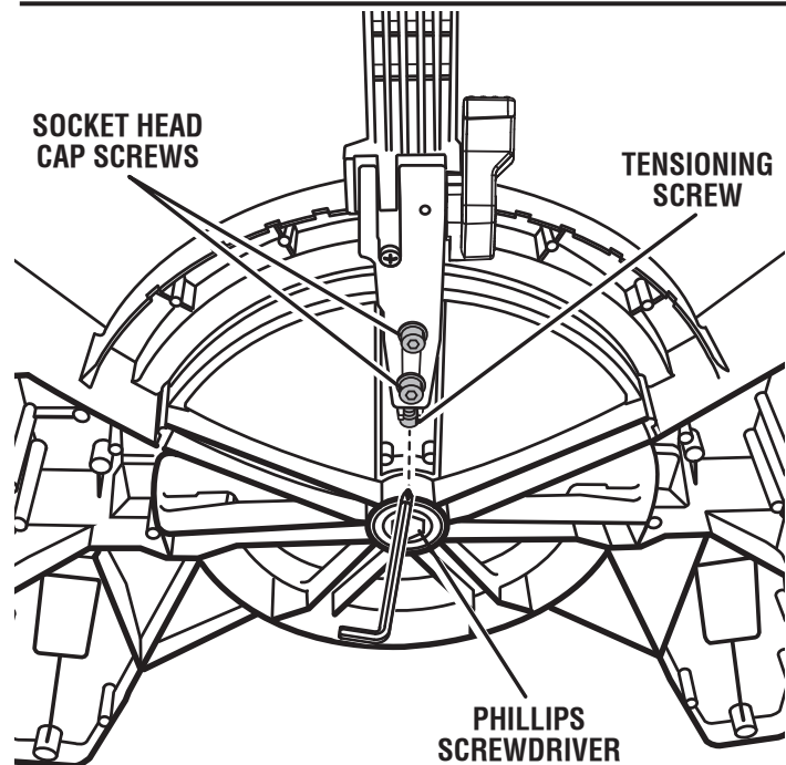
BOTTOM VIEW OF SAW
