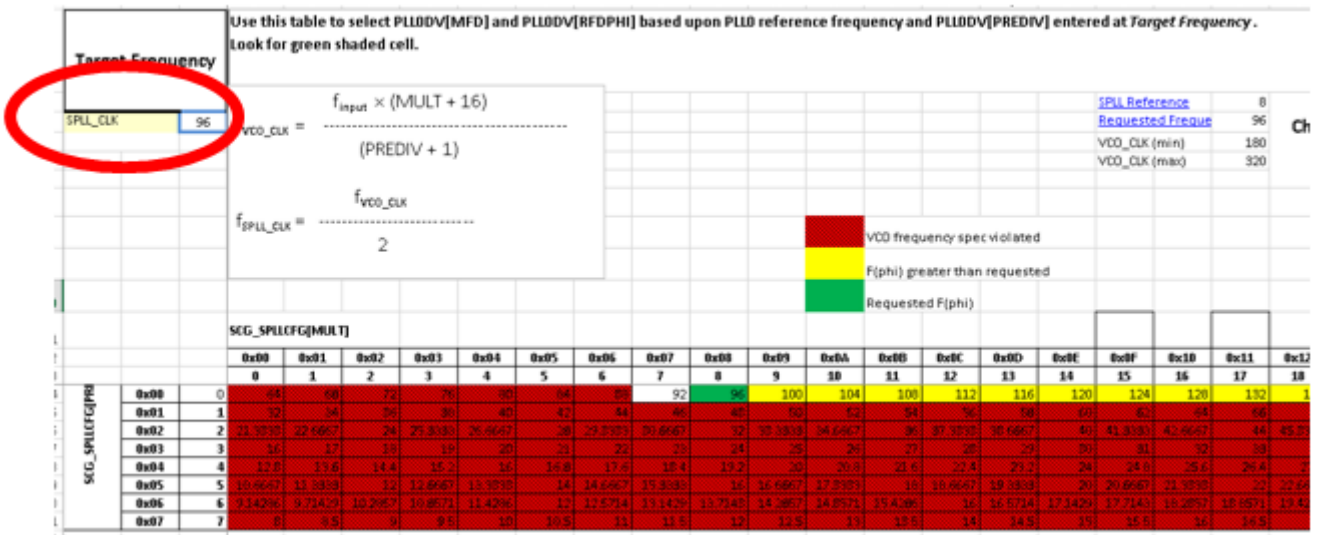
Figure 32. spll_clk table with new settings
