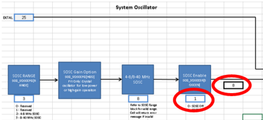
Figure 27. SOSC Turned On
