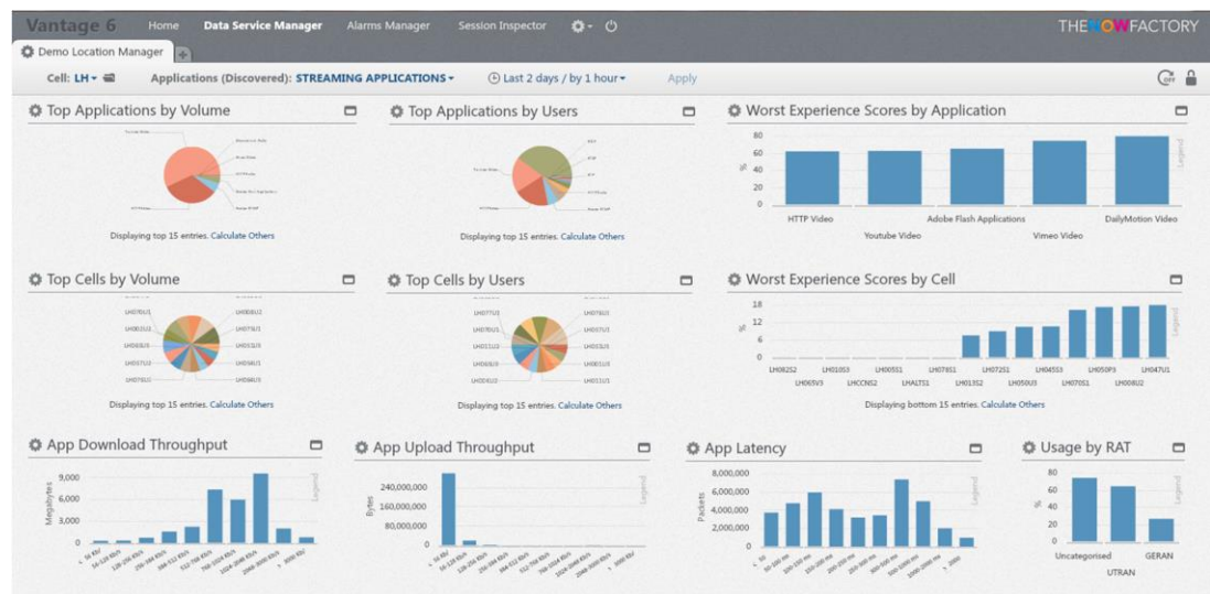
Figure 4: Customer Experience Analytics on Video Streaming Applications
