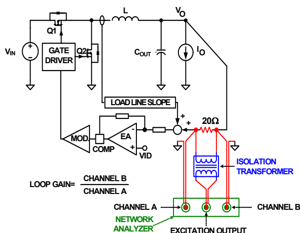
Figure 86. Loop Gain T2(S) Measurement Setup
