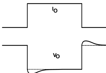
Figure 82. Load Transient Response When C_n is too Small
