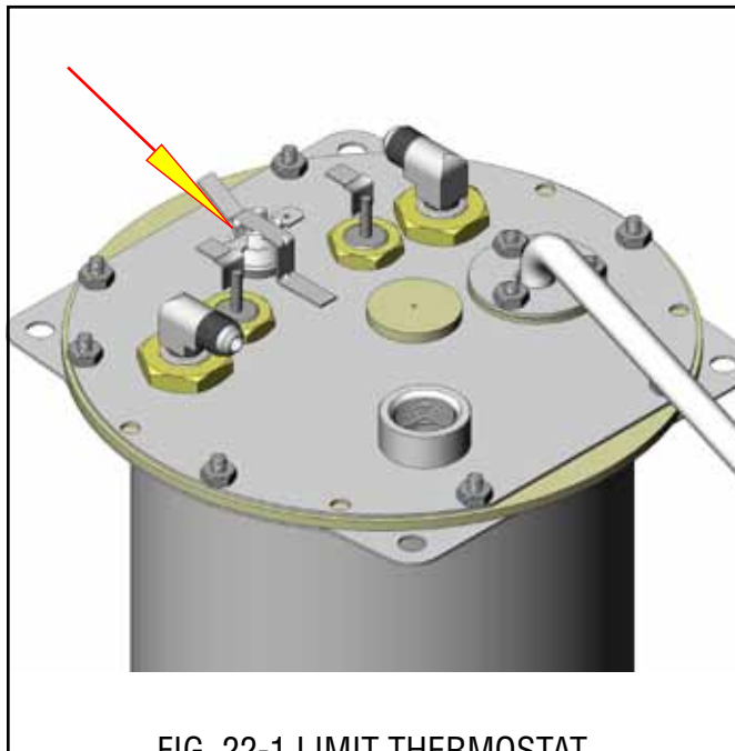
FIG. 22-1 LIMIT THERMOSTAT
