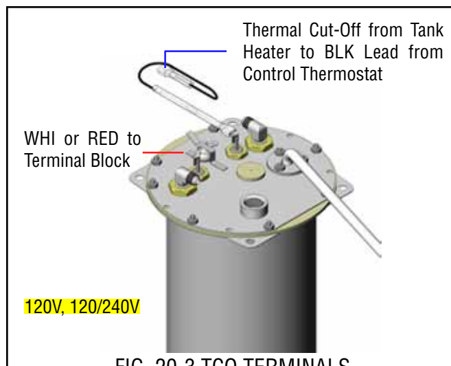
FIG. 20-3 TCO TERMINALS
