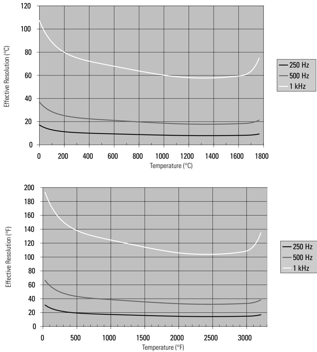
Figure 20 - Effective Resolution versus Input Filter Selection for Type S Thermocouples Using 250, 500, and 1 kHz Filters
