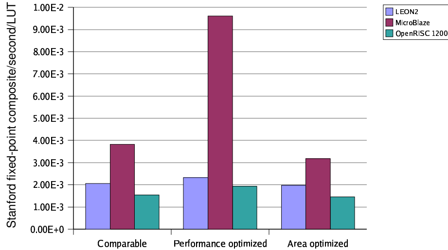
Figure 14: Stanford fixed-point composite/second/LUT for all configurations and processor cores.
