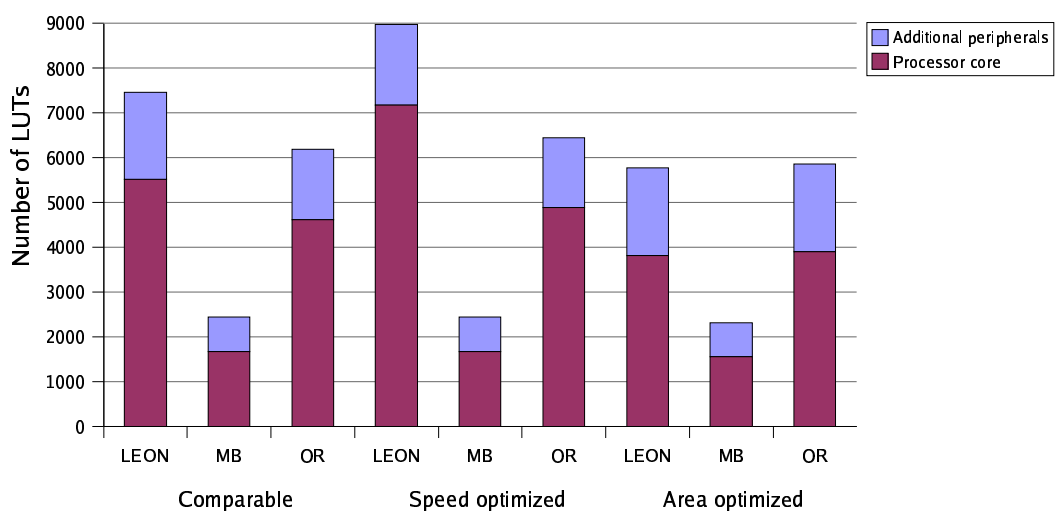
Figure 9: FPGA LUT usage for all processor cores and additional peripherals for all configurations. LEON, MB and OR are abbreviations for LEON2, MicroBlaze and OpenRISC 1200 respectively.
