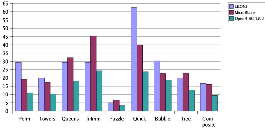
Figure 5: Stanford integer results for the performance optimized configuration. The result is presented in iterations/second.
