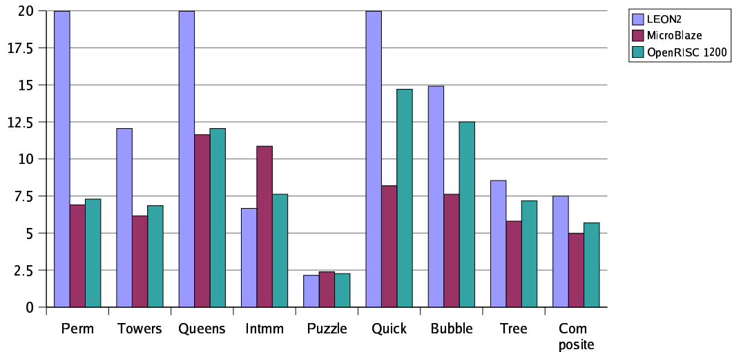
Figure 6: Stanford integer results for the area optimized configuration. The result is presented as iterations/second.
