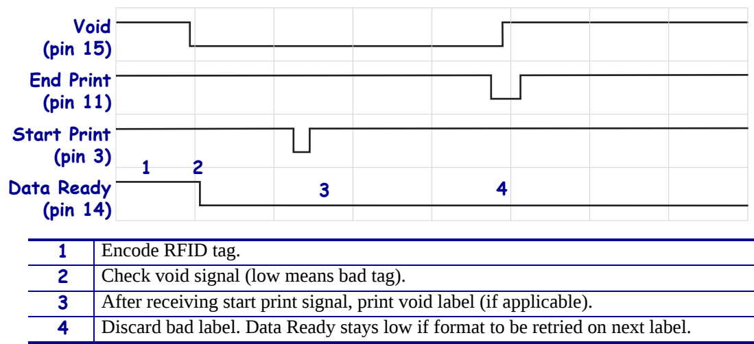
Figure 12 • Single Signal Mode, Bad RFID Tag
