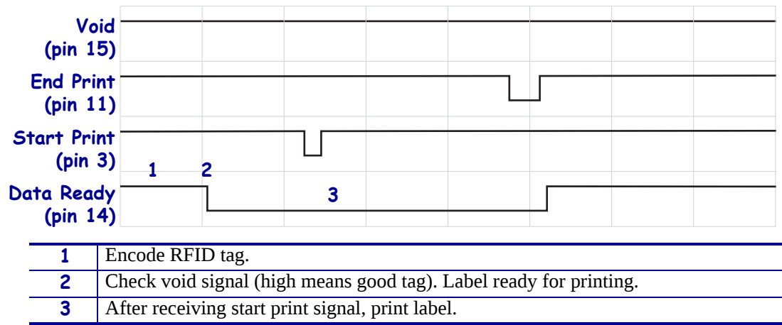
Figure 11 • Single Signal Mode, Good RFID Tag
