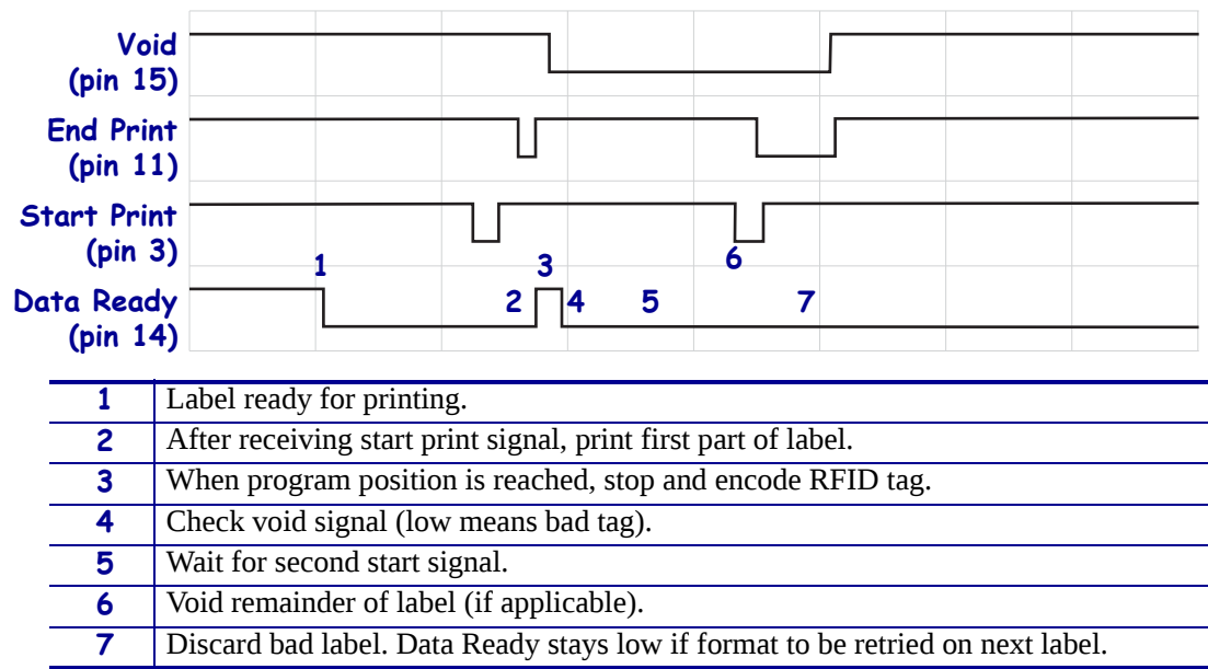
Figure 14 • Double Signal Mode, Bad RFID Tag
