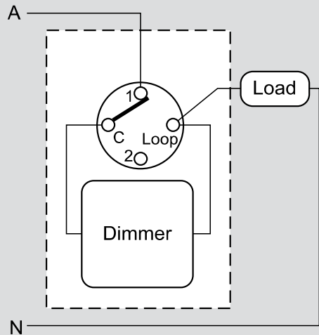
One-way switching with dimmer
