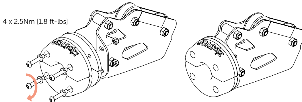
bumpSTOP Assembly
