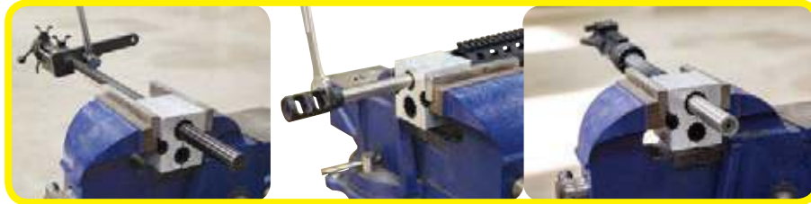
Three different barrel openings of .85", .66" and .53"
