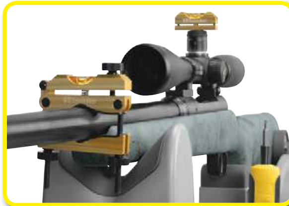
Professional Reticle Leveling System clamshell: 6" wide x 11" high x 3" deep
