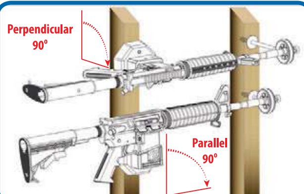
Mag Lock Wall Mount kit includes: steel cable, Mag Lock, Wall Mount, 2 barrel Mount I Bolts
