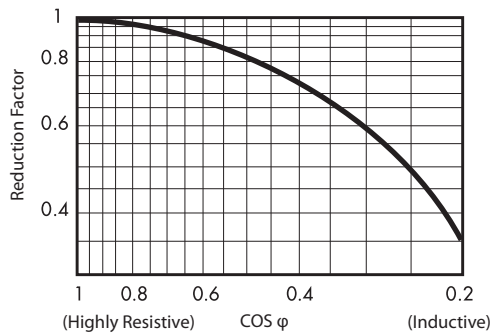
Load Reduction factor versus cos φ
