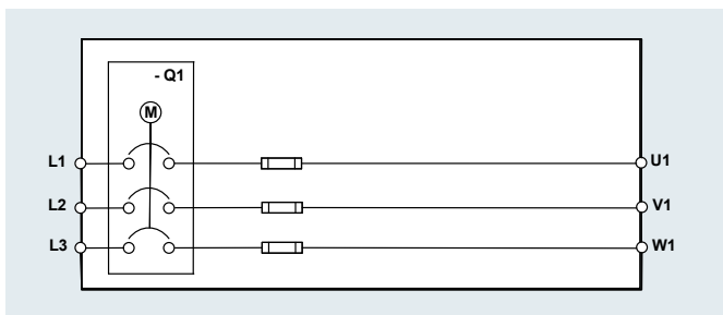
Example of a Line Connection Module for a Smart Line Module
