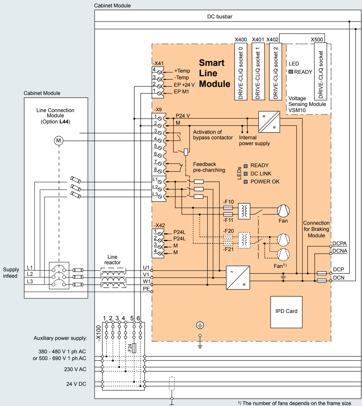
Connection example of a Smart Line Module
