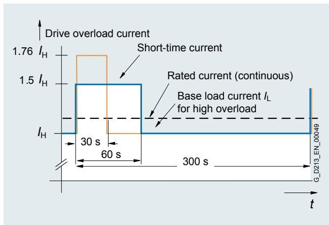
High overload
