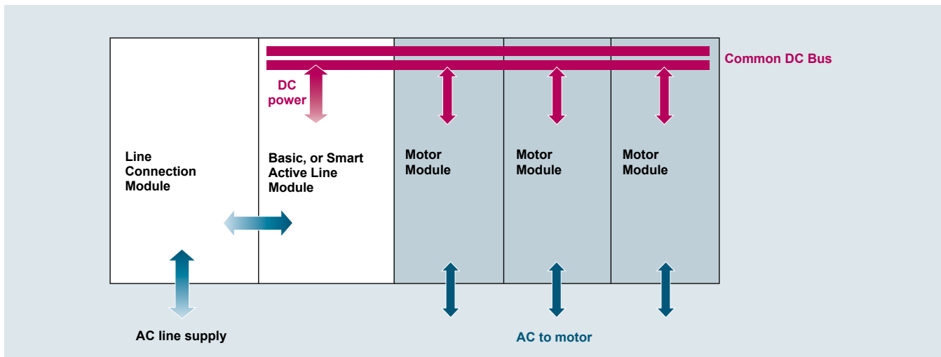
Basic power flow in a SINAMICS S120 Cabinet Module line-up
