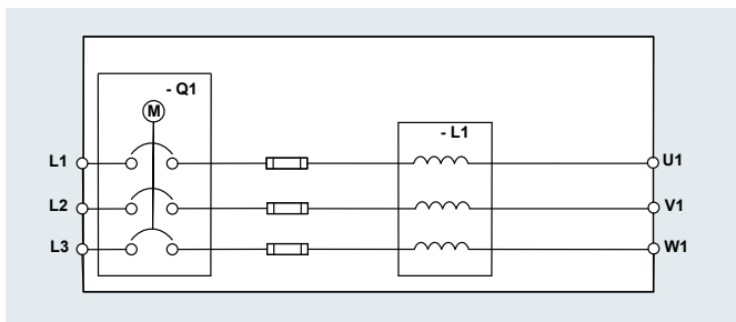
Example of a Line Connection Module for a Basic Line Module
