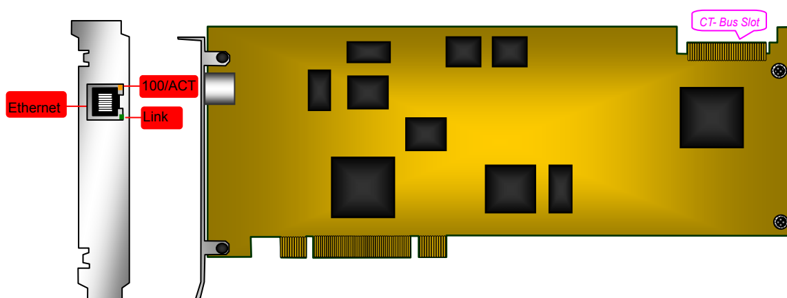
Figure 2-4 Left View & Front View
