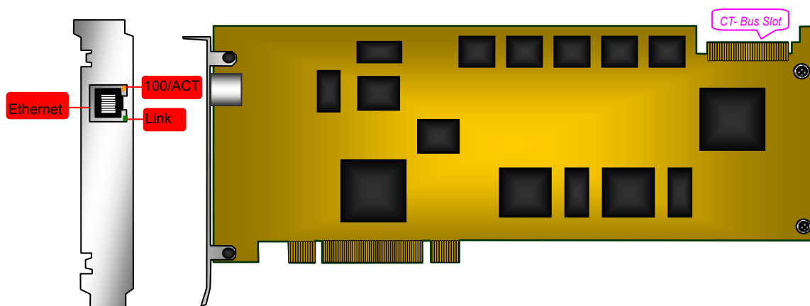
Figure 2-1 Left View & Front View
