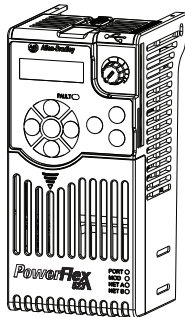
Control module 25A-CTM1
