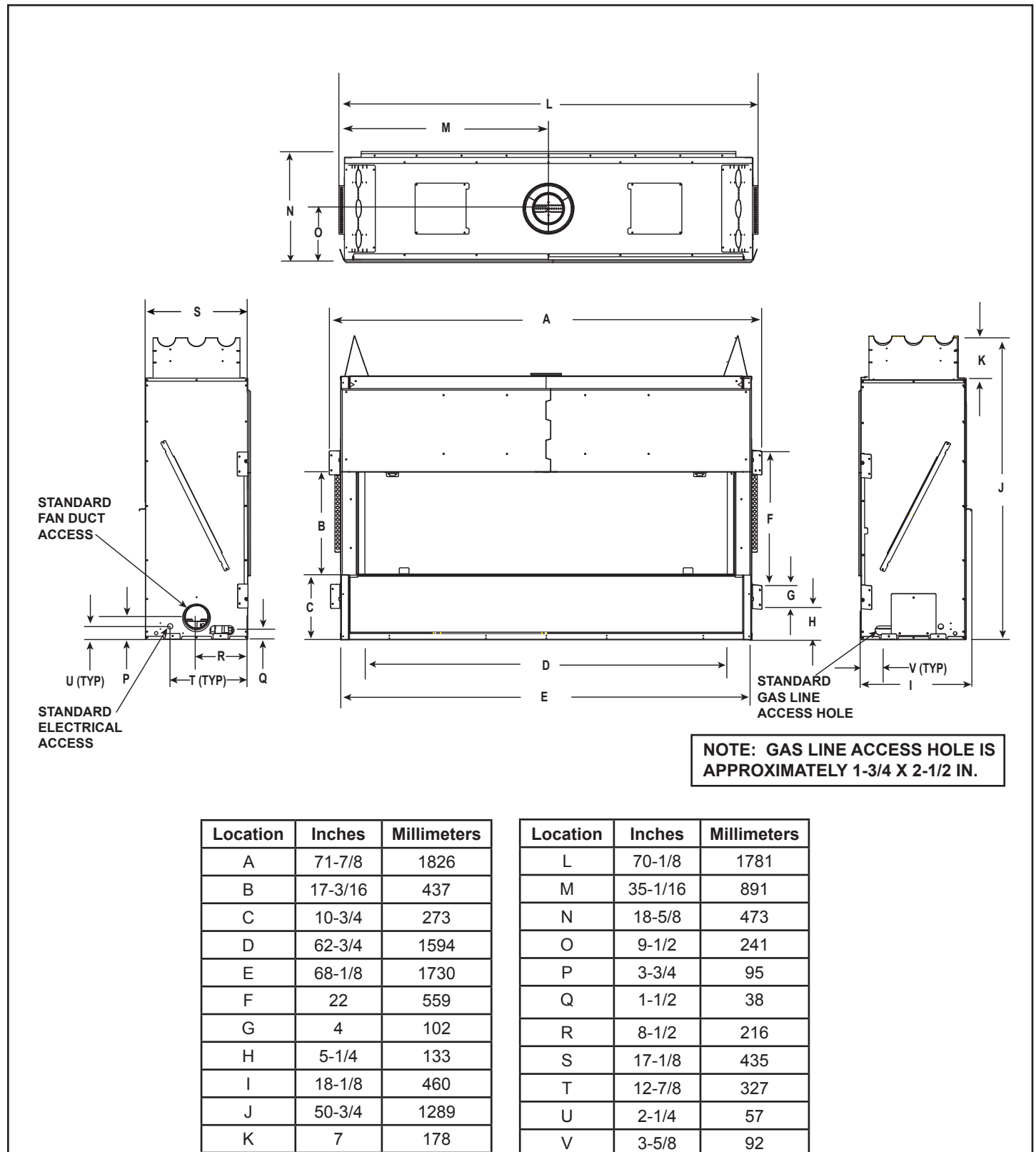
Figure 3.1 Appliance Dimensions
