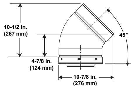
DVP45 (45° Elbow)
