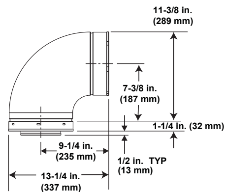
DVP90ST (90° Elbow)
