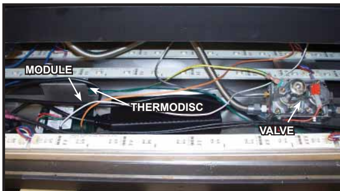
Figure 8.4 Valve Cavity
